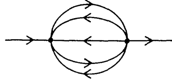
FIG. 2. Graph contributing to baryon dissipation.
